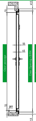
Vertical section/4-sided
