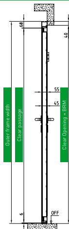
Vertical section/Installation behind opening
