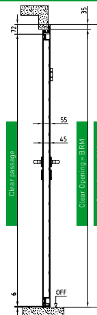
Vertical section/3-sided
