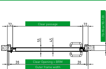
Horizontal section
