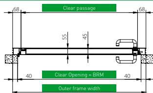
Horizontal section/Installation behind opening
