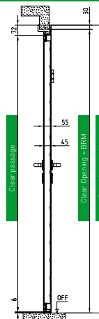
Vertical section
