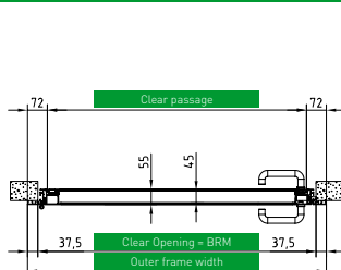
Horizontal section
