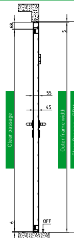
Vertical section/Installation in opening
