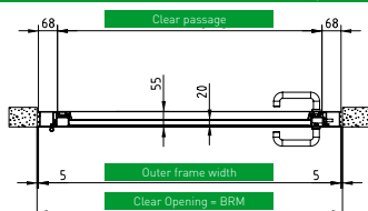
Horizontal section/Installation in opening
